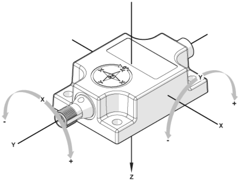
horizontal installation position / rotation about x- and y-axis
