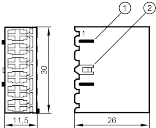
Figure shows contact housing with closed cover 1 View on contact plug-in side 2 Snap spring
