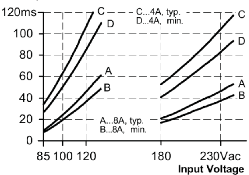
Hold-up Time
