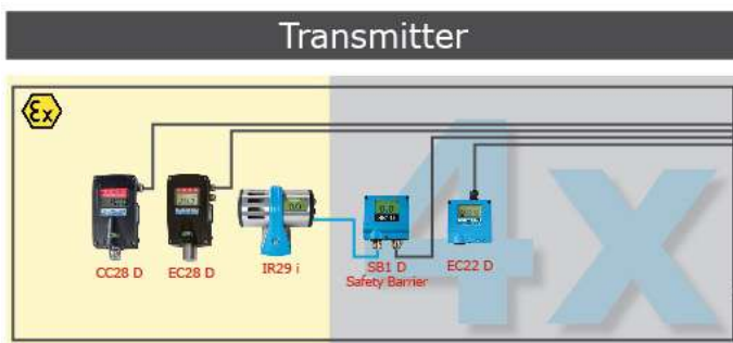
Power of the GMA200-MW4 Controller system.
