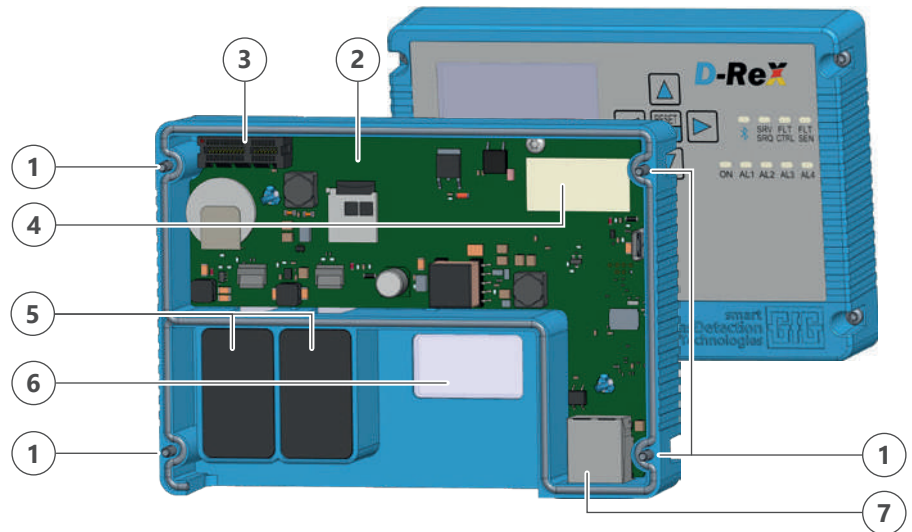
D-ReX housing cover - interior
