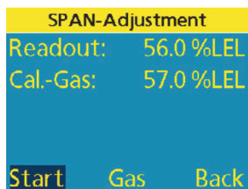
Start SPAN-Adjustment
