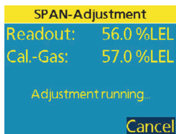
Active SPAN-Adjustment
