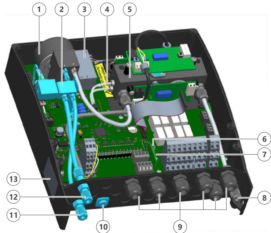
Assemblies GMA200-MGSS/V1
