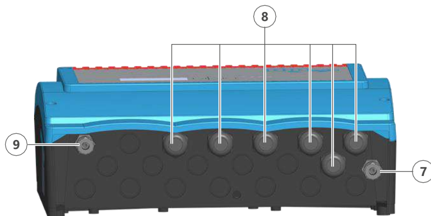
Connections GMA200-MGSS/V0
