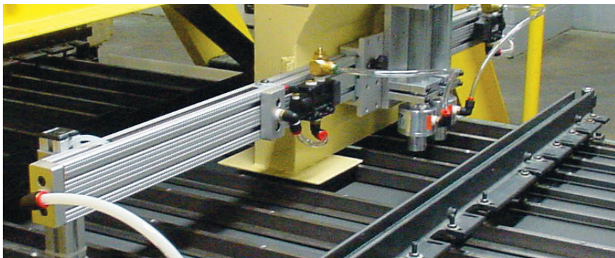
(2) Model 6083 1-1/2" (38mm) Line Vacs convey rejected metal caps from a fluorescent lamp operation to a scrap bin.
