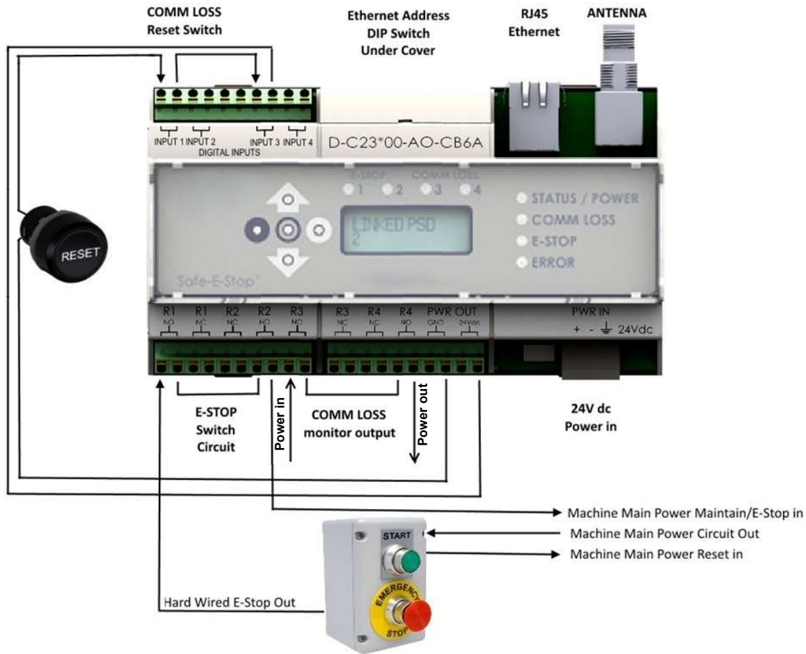
Figure 13: MSD Typical Single Channel Connections When Not Using the COMM LOSS Relays
