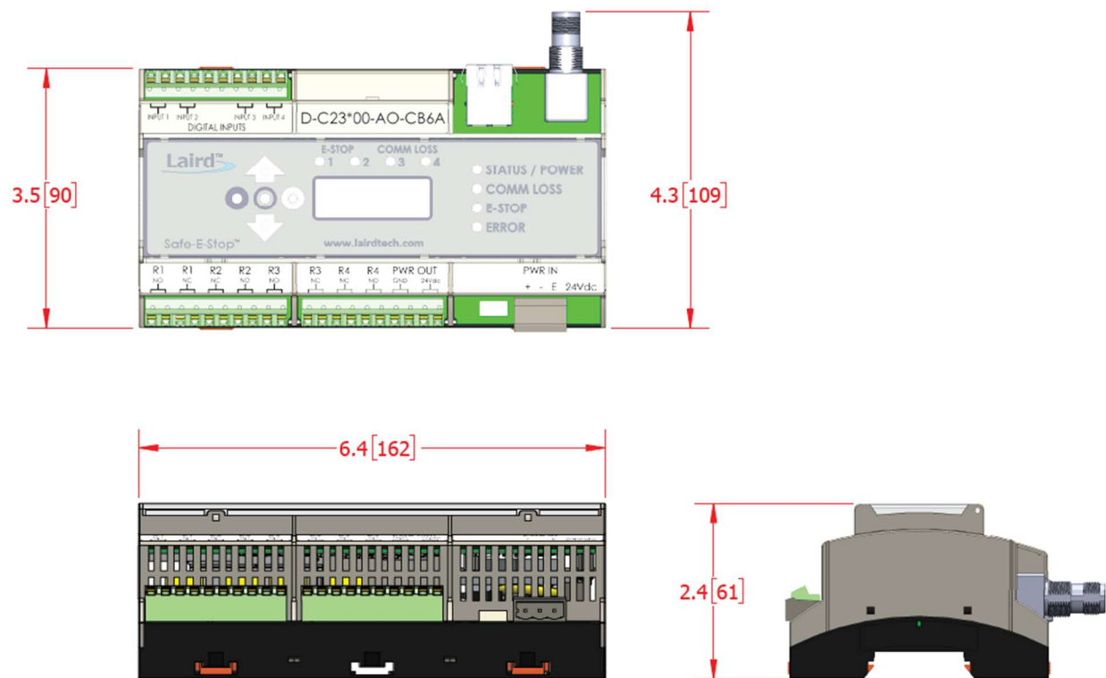
Figure 21: MSD Dimensions
