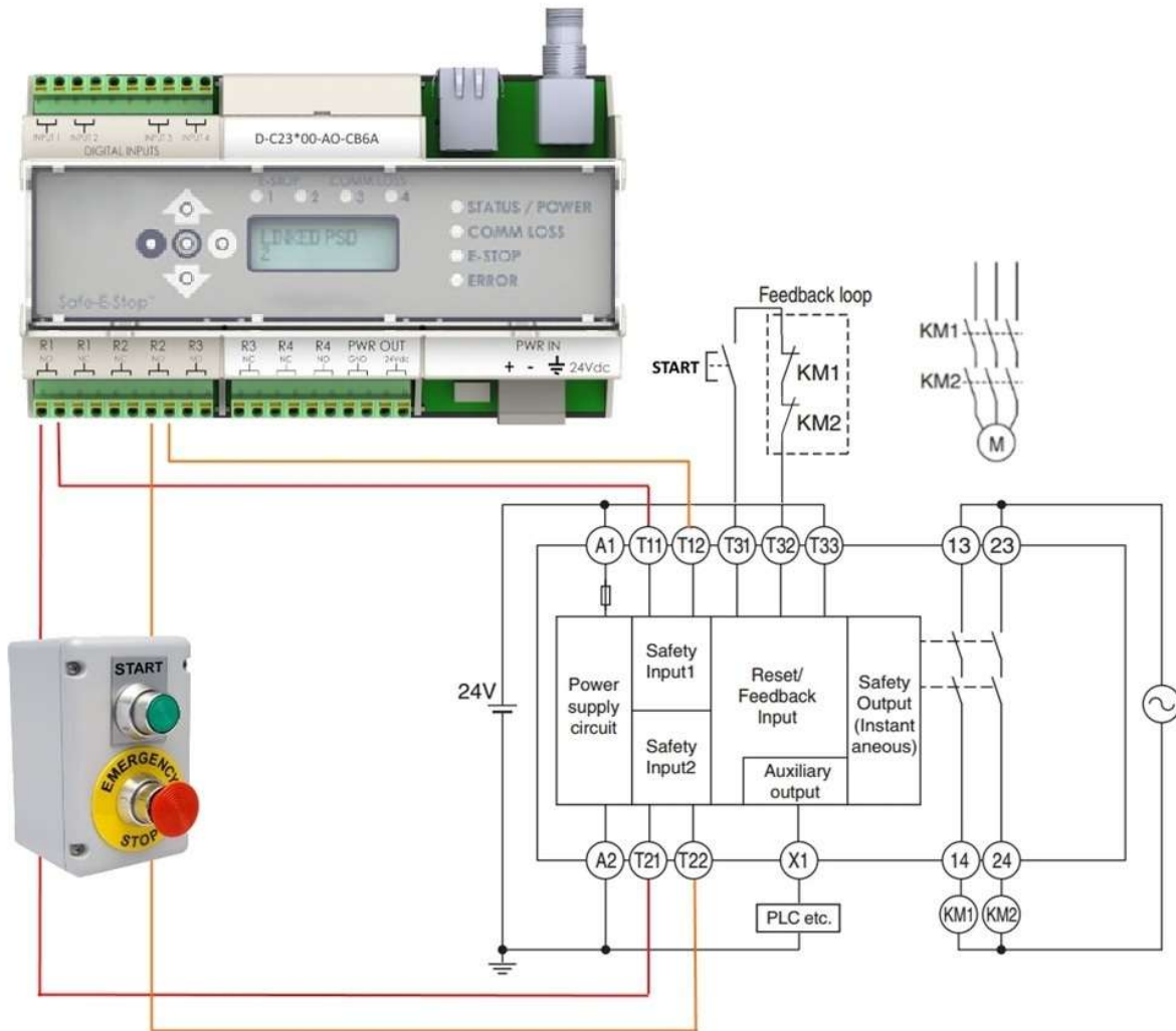
Figure 14: MSD Typical Dual Channel Connections When Not Using the COMM LOSS Relays
