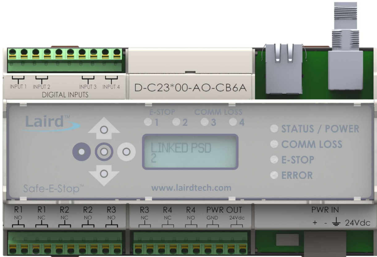
Figure 16: MSD Status Indicators
